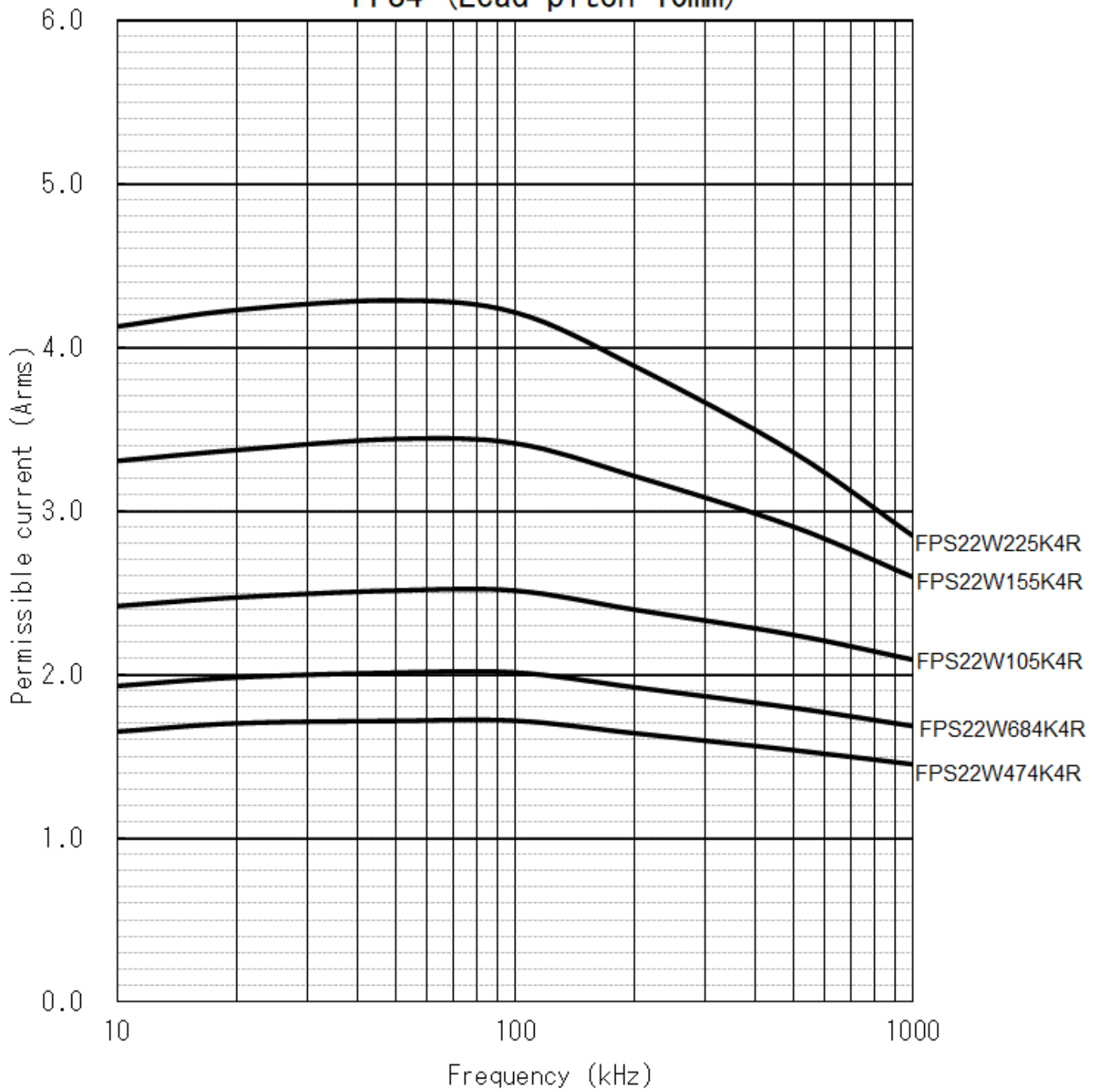
Permissible current (Effective value) VS Frequency FPS4 (Lead pitch 10mm)
