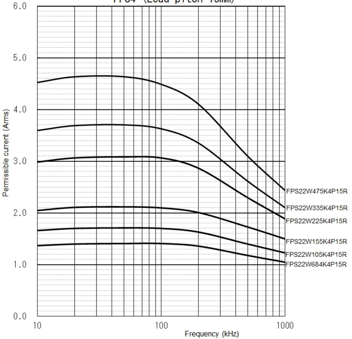
Permissible current (Effective value) VS Frequency FPS4 (Lead pitch 15mm)
